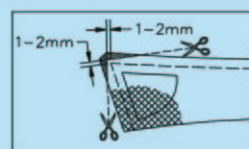
Trimming excess margin of collar point 切除多餘的領尖止口
