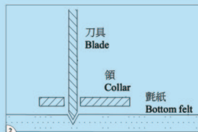
跟機件: Standard: 直刀片 Straight Cutting Blade
