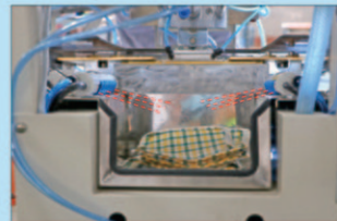
特殊除静电装置，可消除布料产生的静电，使收料效果更佳 With special anti-static device to offset static electricity generated by fabrics to facilitate collection in neatly manner
